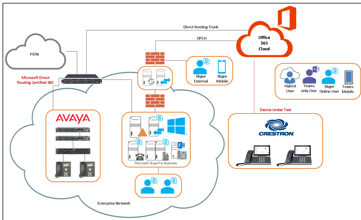
Figure 1 Network Topology
