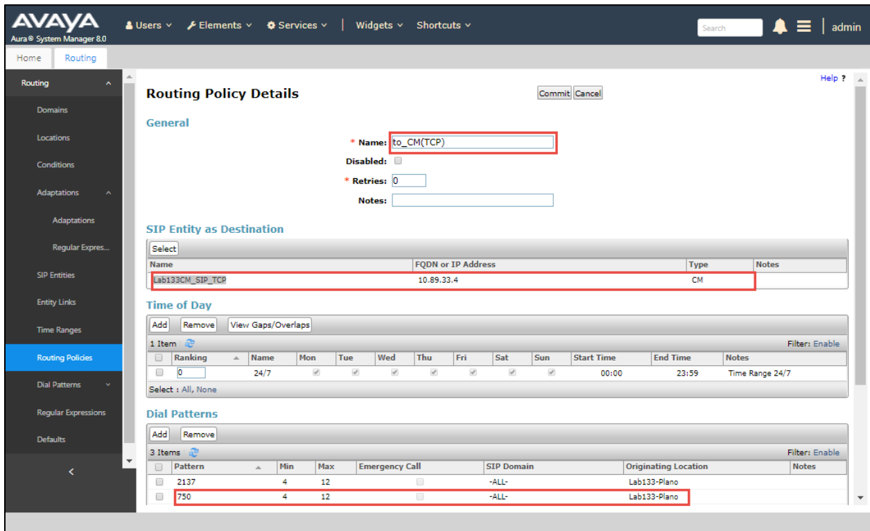
Figure 153 - Routing Policy to Avaya Aura Communication Manager
